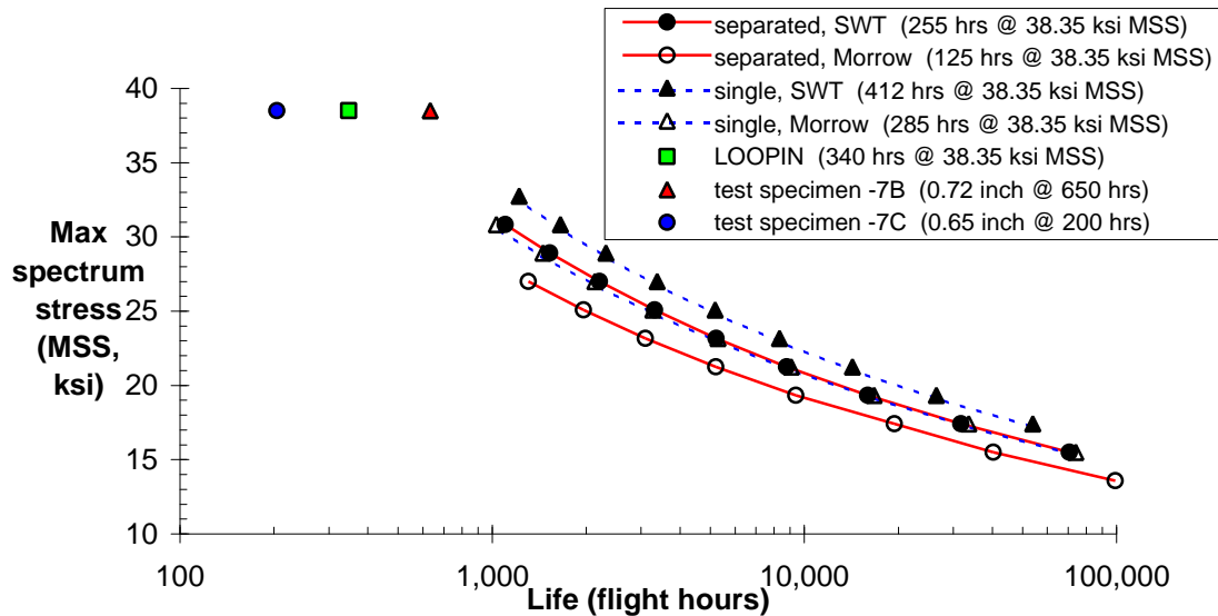
Figure 14. MSC/FATIGUE, LOOPIN, and test results - F-16 479 bulkhead
