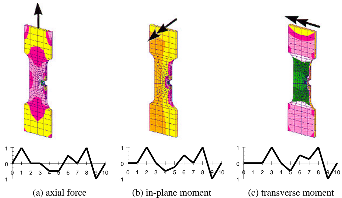
Figure 5. Finite element models (with results) and corresponding loading histories for combined loading of three-dimensional semi-circular edge notch geometry
