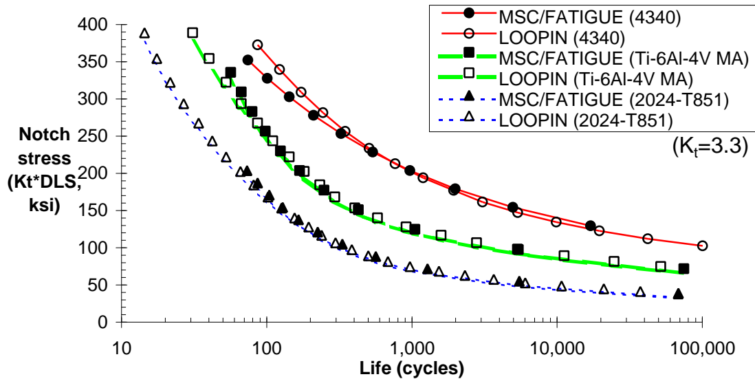
Figure 3. MSC/FATIGUE and LOOPIN results - hole specimen, constant amplitude
