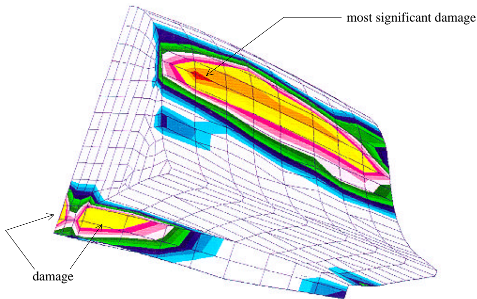
Figure 15. MSC/FATIGUE results - forward fuselage / fuel tank life contour plot
