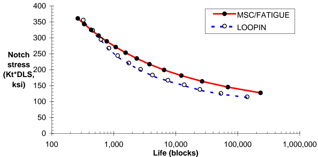
Figure 6. MSC/FATIGUE and LOOPIN results - combined loading example
