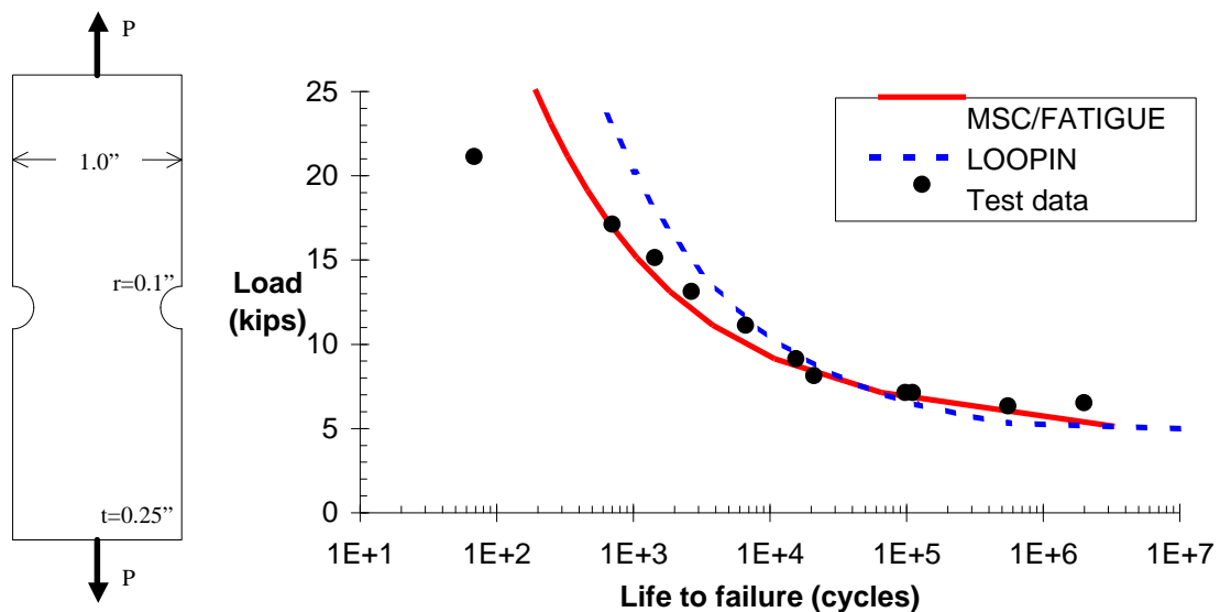
Figure 8. MSC/FATIGUE, LOOPIN, and test results - blunt edge notch specimen [7]
