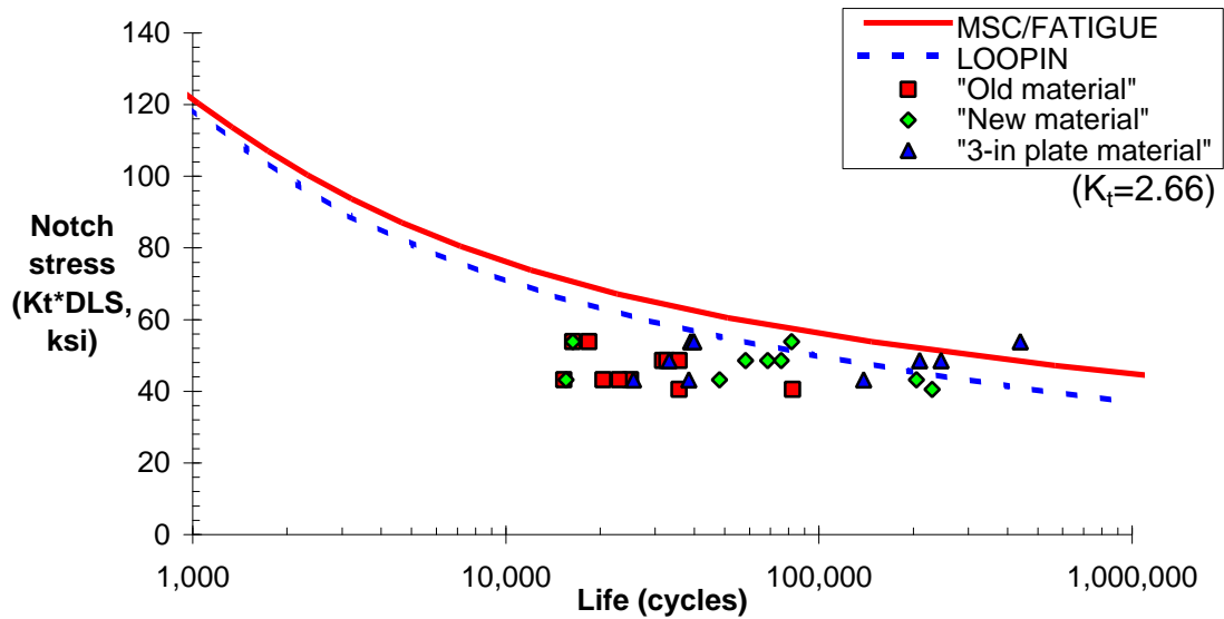
Figure 7. MSC/FATIGUE, LOOPIN, and test results - Purdue/ALCOA specimen [6]
