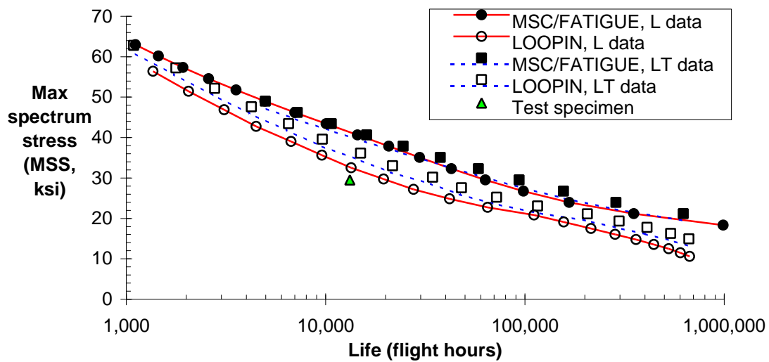
Figure 11. MSC/FATIGUE and test results - Shear web beam
