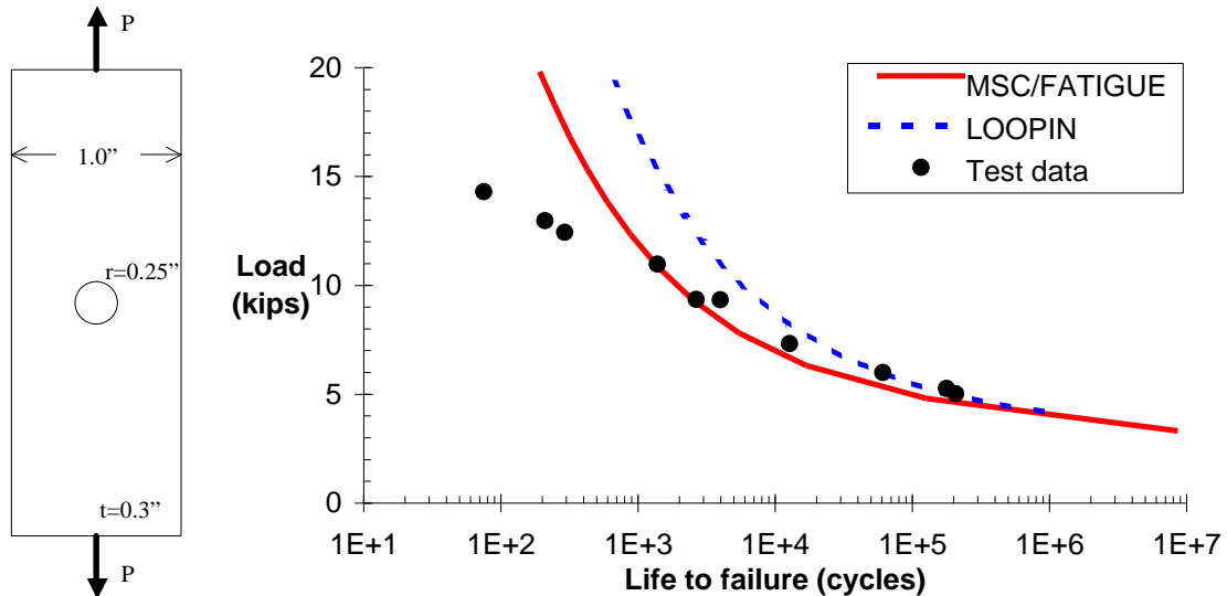
Figure 9. MSC/FATIGUE, LOOPIN, and test results - center hole specimen [7]
