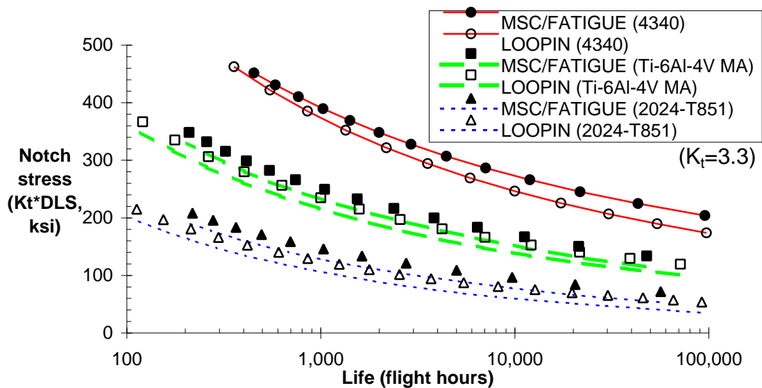
Figure 4. MSC/FATIGUE and LOOPIN results - hole specimen, FALSTAFF
