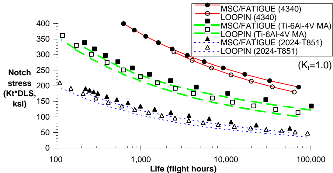
Figure 2. MSC/FATIGUE and LOOPIN results - smooth specimen, FALSTAFF
