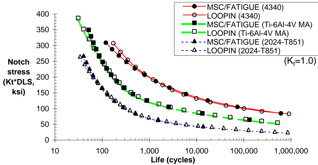
Figure 1. MSC/FATIGUE and LOOPIN results - smooth specimen, constant amplitude
