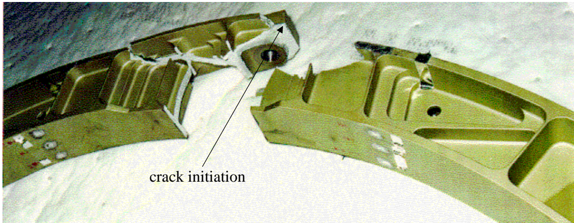
Figure 12. F-16 479 bulkhead test specimen number -7B, post-failure [8]
